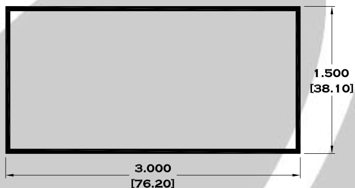
11084 TUBO RECTANGULAR DE 3" X 1 1/2"
