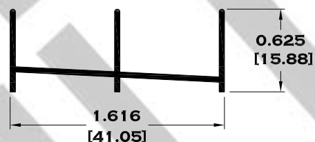
9524 GUIA
