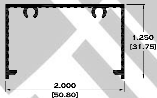
8591 BOLSA LISA
