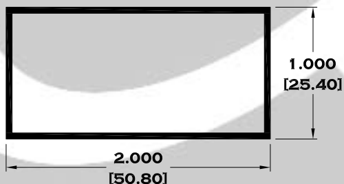
11121 TUBO RECTANGULAR DE 2" X 1"
